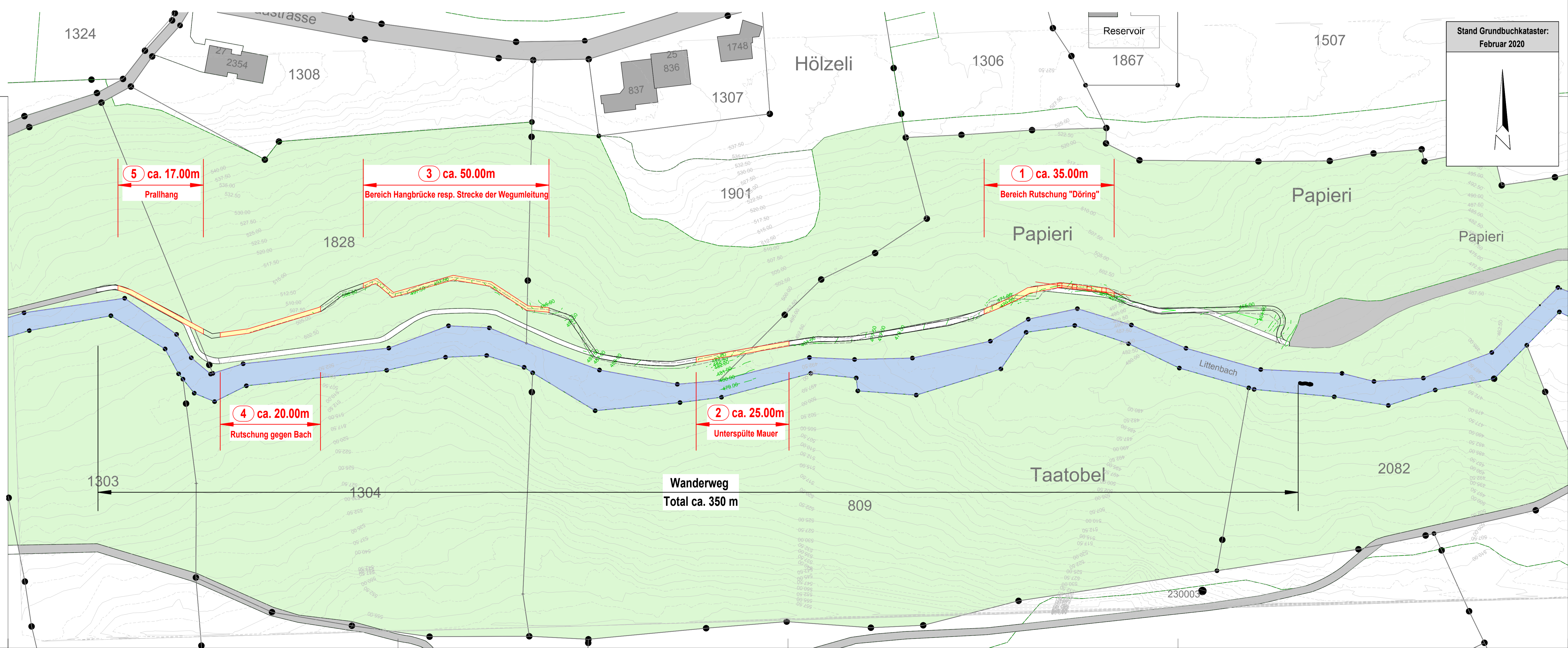
Situation, 1:500
